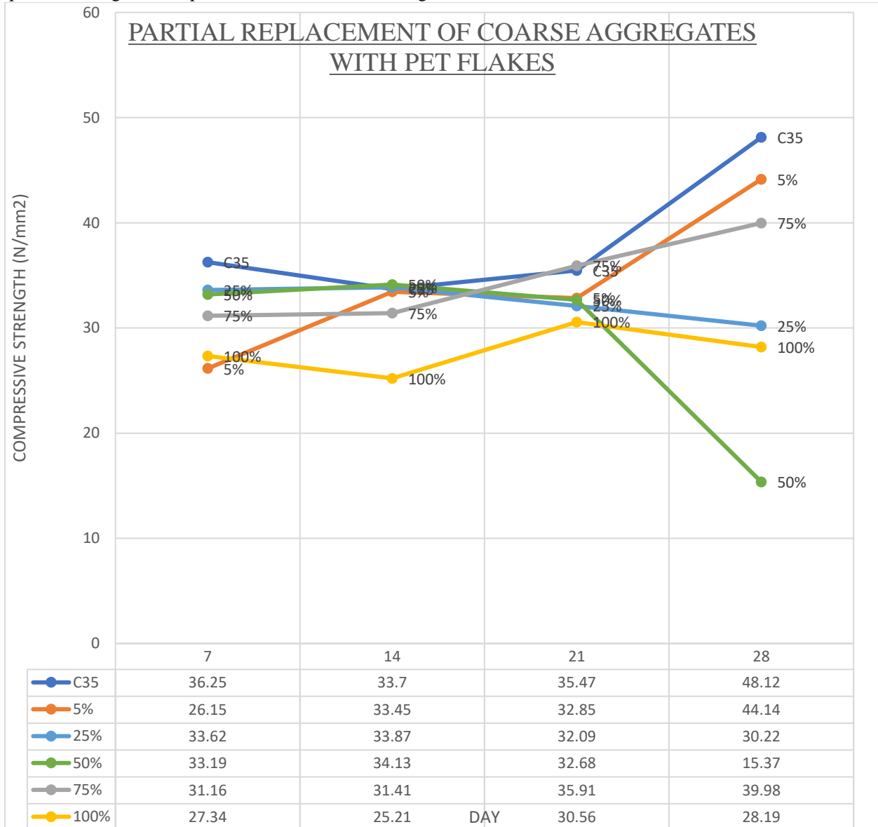
Fig 6: Compressive strength
