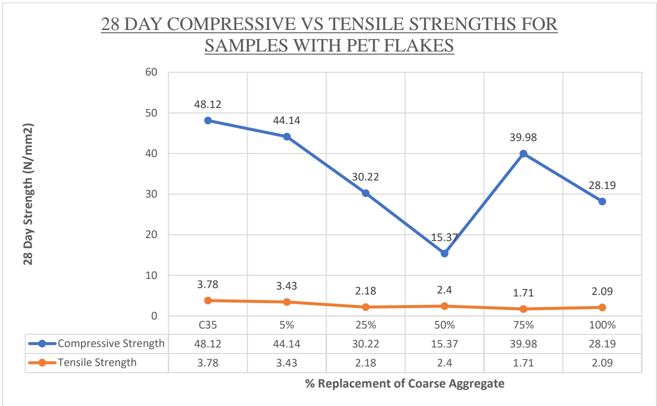
Fig 7: Compressive strength vs. Tensile strength.
