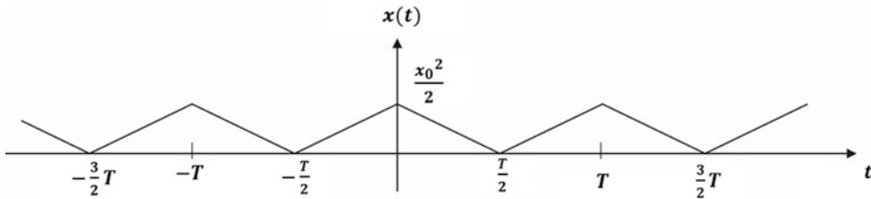
Fig. 22.15 Autocorrelation function R(\tau) for the function of Illustrative Example 22.2
