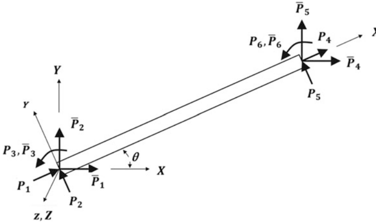
Fig. 11.6 Beam element showing nodal forces P_i in local (x, y, z) and nodal forces \bar{P}_i , in global coordinate axes (X, Y, Z)
