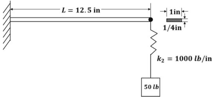
Fig. 1.8 System for Illustrative Example 1.2
