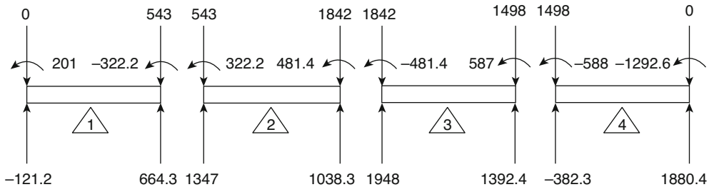
Fig. 10.14 Dynamic equilibrium for beam element of Illustrative Example 10.6
