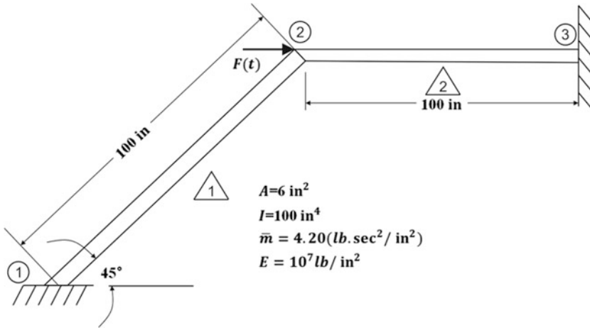
Fig. 11.7 Plane Frame of Illustrative Example 11.1
