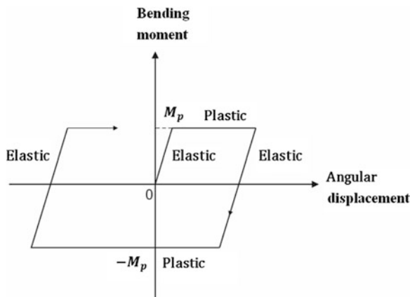
Fig. 16.6 Elastoplastic relationship between bending moment and angular displacement at a section of a beam
