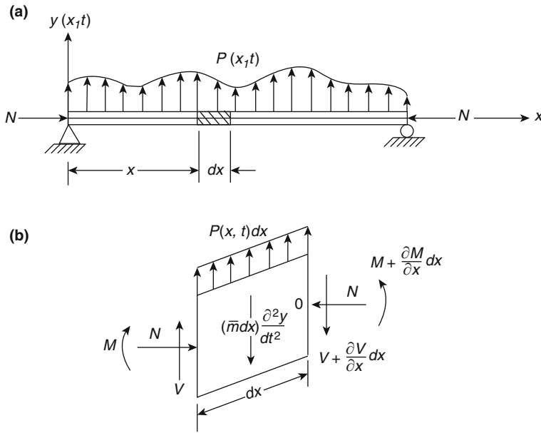
Fig. 18.4 Beam supporting constant axial force and lateral dynamic load. (a) Loaded beam. (b) Forces acting on a differential element
