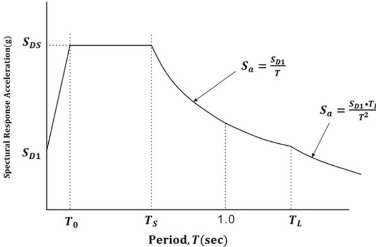
Fig. 24.1 Design response spectrum plot
