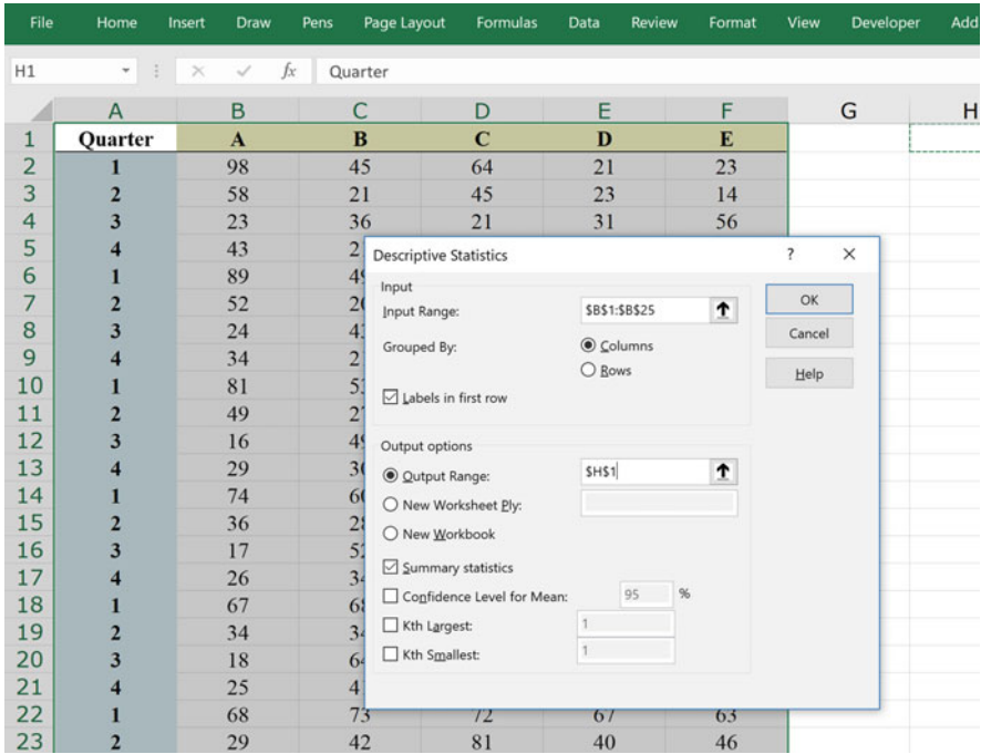
Fig. 3.12 Dialog box for descriptive statistics
