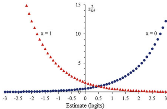
Fig. 15.1 Squared standardized residuals for a dichotomous item of difficulty 0.5
