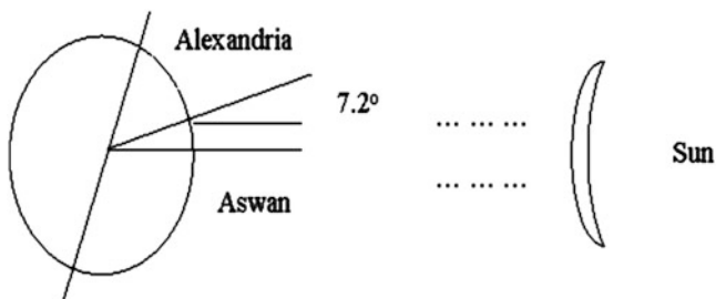
Fig. 1.6 Eratosthenes measurement of the circumference of the earth
