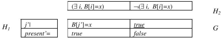
Fig. 16.4 Finding Index in Array
