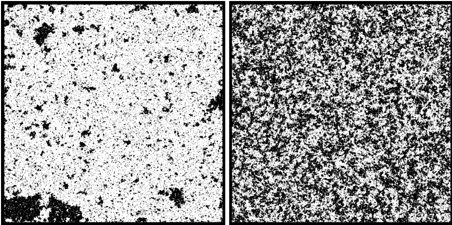
Fig. 18.5 Equilibrium states of the Ising model on an 800 \times 800 grid (black dot = spin +1). Left side: below the critical temperature ( \beta > \beta_c ); Right side: above the critical temperature
