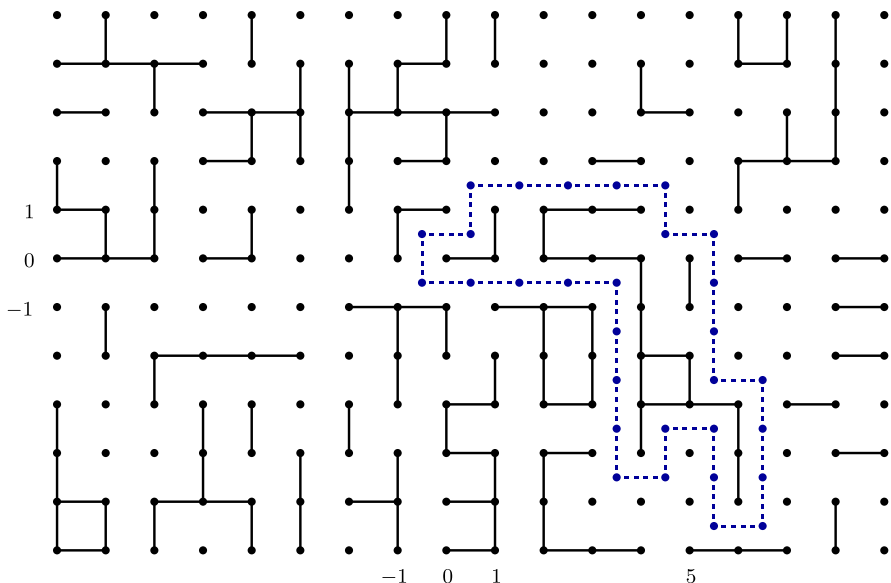
Fig. 2.2 Contour of the cluster C_5
