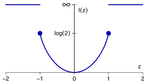
Fig. 23.1 Rate function I(z) from (23.6)
