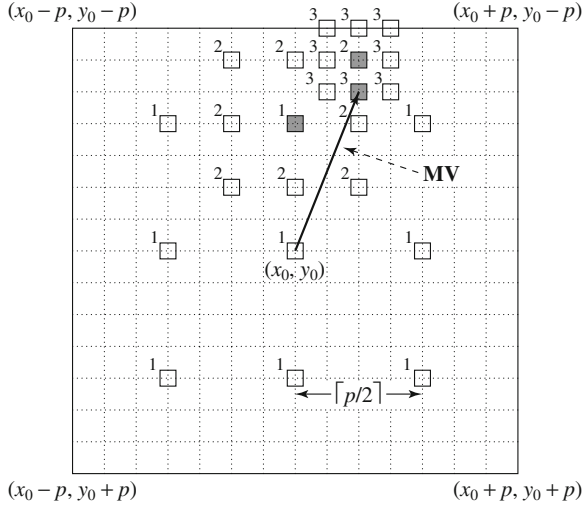
Fig. 10.2 2D Logarithmic search for motion vectors
