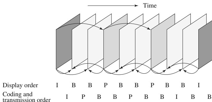
Fig. 11.3 MPEG frame sequence
