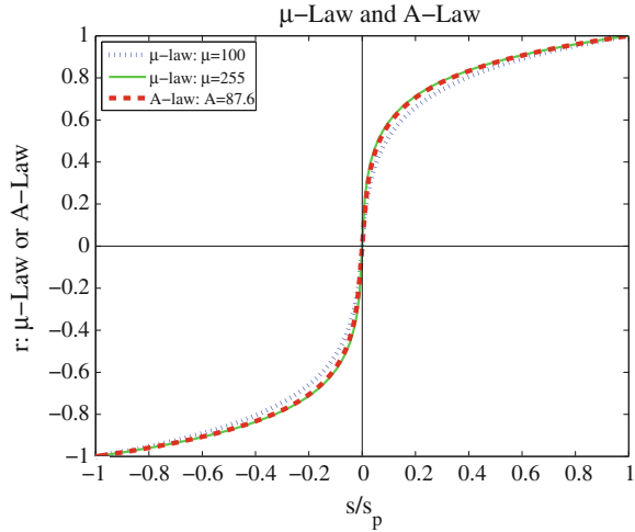
Fig. 6.6 Nonlinear transform for audio signals
