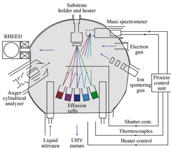
FIGURE 28.5. Molecular beam epitaxy system.
