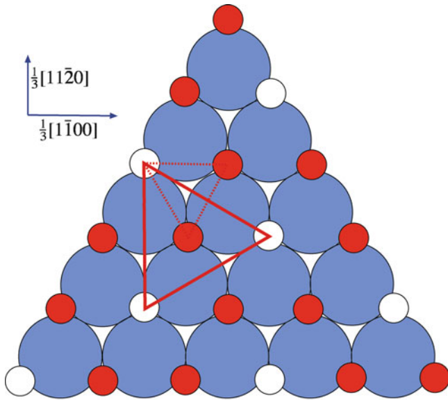
FIGURE 12.12. Schematic shows b of perfect dislocations in \text{Al}_2\text{O}_3 .
