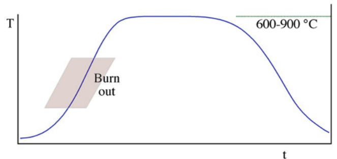
FIGURE 27.16. Typical thick film circuit firing profile.
