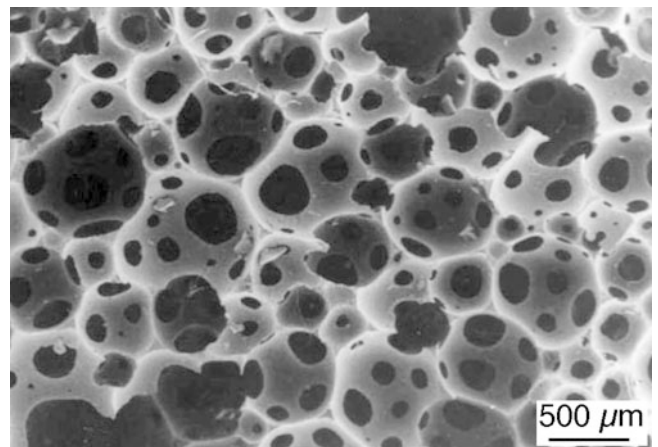
FIGURE 15.15. Sintered alumina foam made using a soap-nut slurry with 40 vol. % ceramic.
