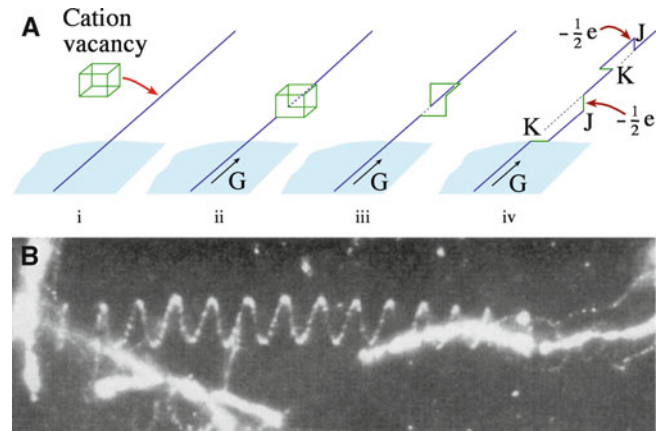
FIGURE 12.18. Forming a pair of kinks and a pair of jogs and how this leads to helical dislocations in MgO.
