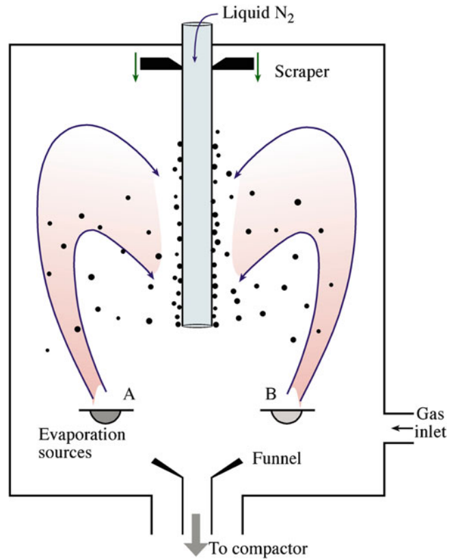
FIGURE 20.8. Gas-condensation chamber for nanoparticle synthesis.
