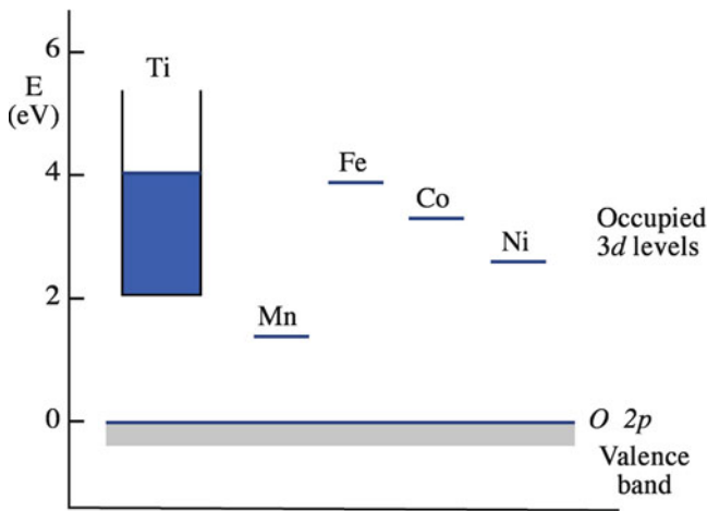
FIGURE 30.7. Electronic energy levels of some 3d monoxides, deduced from spectroscopic measurements. The energy zero has been taken as the top of the oxygen 2p valence band.
