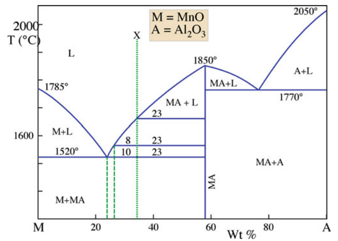
FIGURE 8.22. \text{MnO} – \text{Al}_2\text{O}_3 phase diagram.
