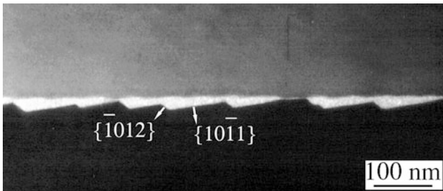
FIGURE 14.30. Intergranular film in \text{Al}_2\text{O}_3 that was initially uniformly thick but varied in thickness after heat treatment.
