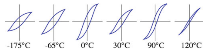
FIGURE 31.13. Hysteresis loops for BaTiO 3 as a function of temperature.
