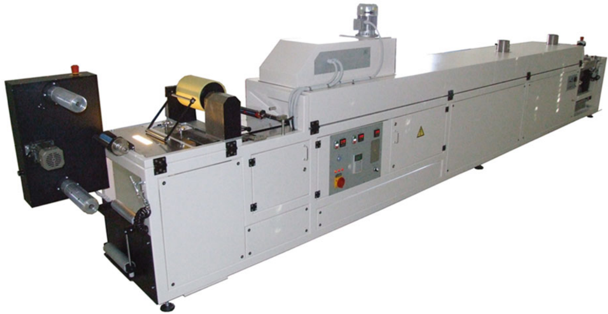
FIGURE 27.4. Example of an industrial tape casting machine.
