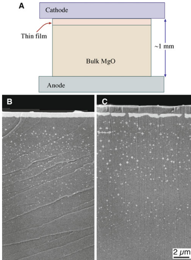
FIGURE 25.23. Reaction between a thin film of \text{Fe}_2\text{O}_3 and a layer of MgO in an electric field at 1,150^\circ\text{C} for 2 h. (A) The setup. (B) Field with nothing applied. (C) Field with 2 kV/cm applied. The MgO has grown on top of the spinel. The reaction is fastest at GBs in the thin film.
