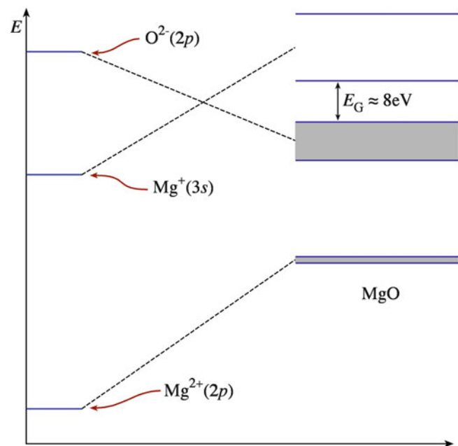
FIGURE 30.23. Energy band diagram for \text{MgO} .
