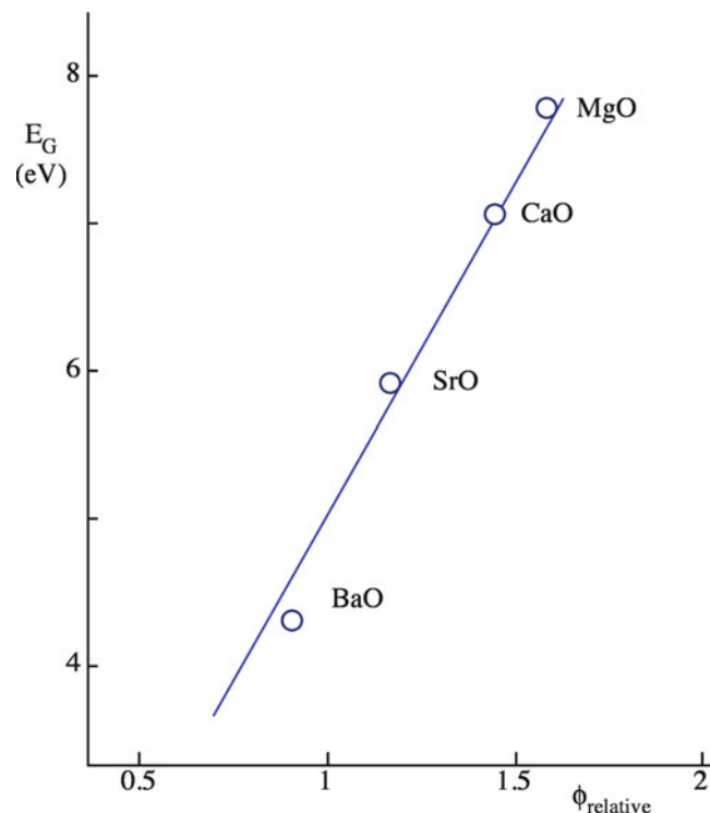
FIGURE 30.24. Effect of bond ionicity on E_g for metal oxides \text{MO} ( \phi = Z/r ).
