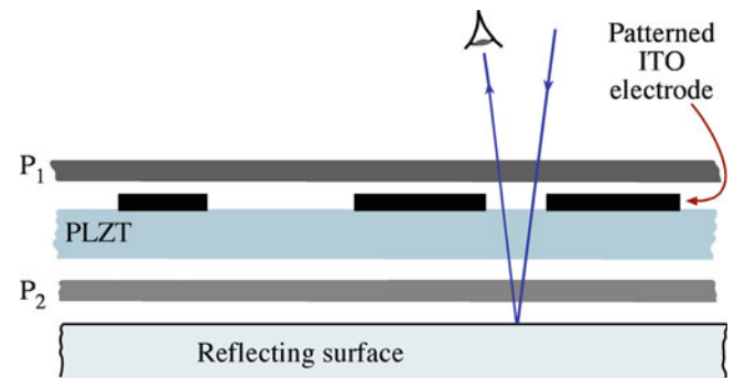
FIGURE 32.24. Basic layout of a PLZT reflective display.
