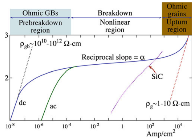
FIGURE 30.17. Typical current–voltage ( I - V ) characteristics for a ZnO varistor.
