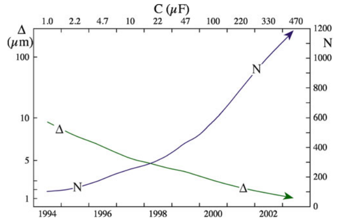
FIGURE 38.4. Trends in number ( N ) of dielectric layers and thickness ( \Delta ) of the dielectric layer.
