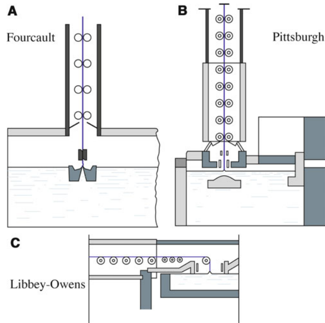
FIGURE 26.8. Drawing processes for window glass. (A) Fourcalt. (B) Pittsburgh. (C) Libbey-Owens.
