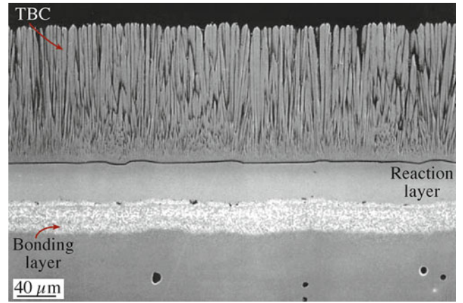
FIGURE 25.3. Technical application 3. Thermal barrier coating on a metal with a reaction layer and a bonding layer.
