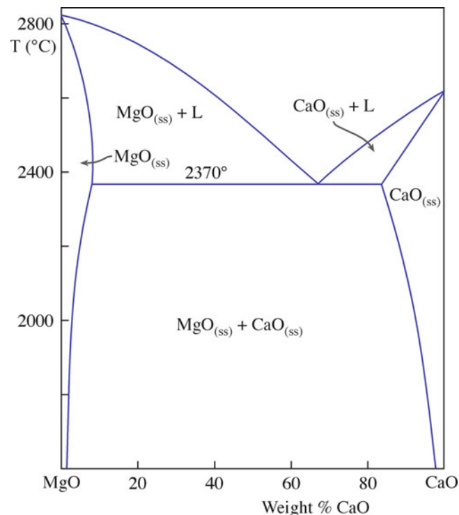
FIGURE 8.11. The MgO–CaO phase diagram.
