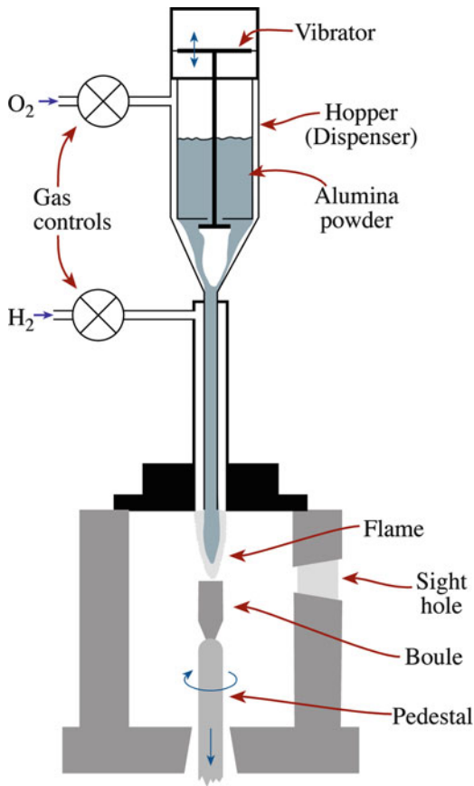
FIGURE 29.1. Verneuil technique.
