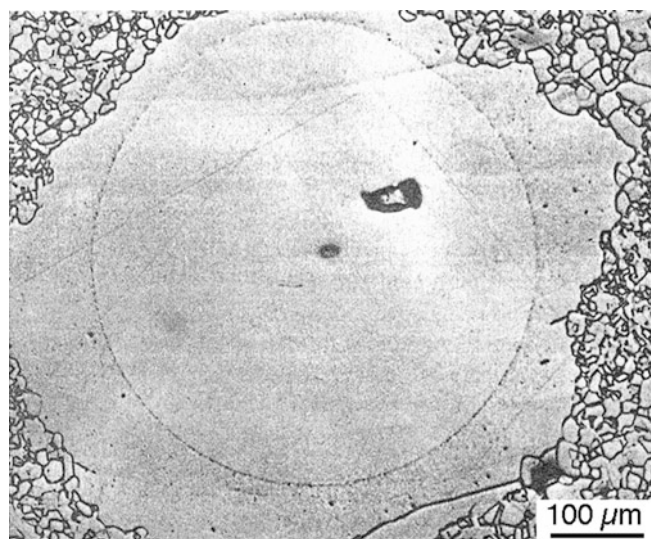
FIGURE 24.22. Using a single-crystal sphere to model exaggerated grain growth in \text{Al}_2\text{O}_3 doped with 1 wt.% \text{MgO} at 1,800^\circ\text{C} for 60 min.
