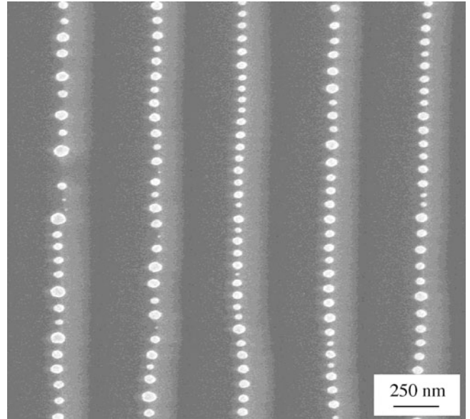
FIGURE 13.28. Self-assembly of Pt nanoparticles due to charging along a surface ridge in \text{Al}_2\text{O}_3 . The particles sit on the ridge, not in the valley!
