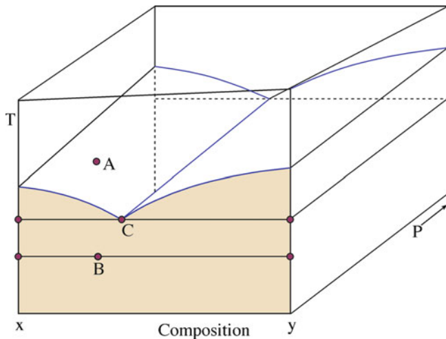
FIGURE 8.9. Model binary phase diagram showing T , P , and composition as variables.
