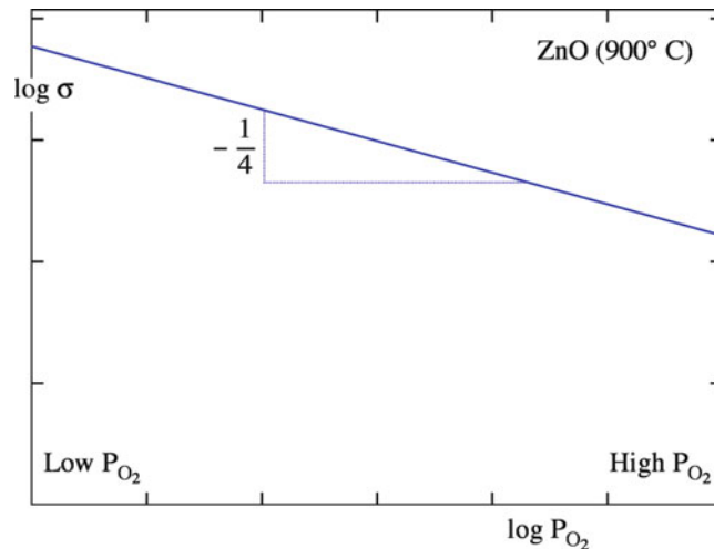
FIGURE 30.13. Effect of oxygen pressure on electrical conductivity of ZnO.
