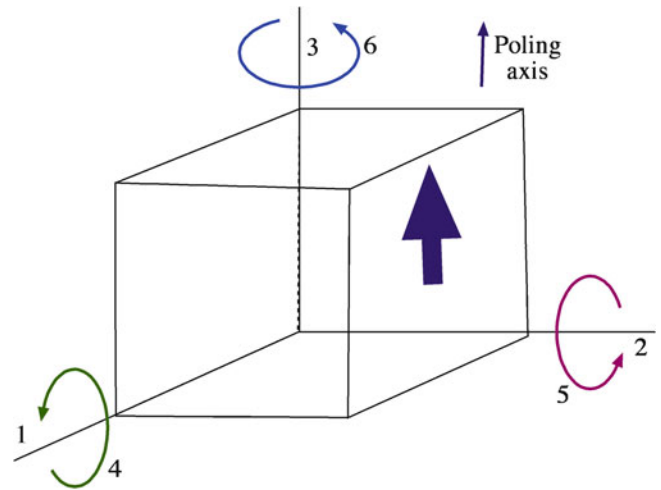
FIGURE 31.19. Notation of axes for piezoelectric ceramic.
