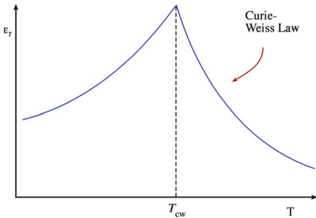
FIGURE 31.6. Relative permittivity of a ferroelectric as a function of temperature.
