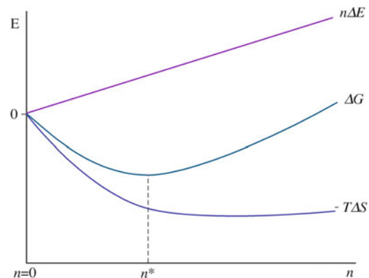
FIGURE 11.3. How the free energy decreases to a minimum as the number of vacancies increases.
