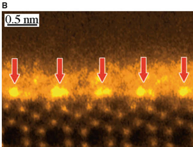
FIGURE 14.27. HRTEM images of intergranular films (IGFs) in \text{Si}_3\text{N}_4 . (A) Phase contrast image. (B) Z-contrast image showing ordering of rare-earth dopant at the glass/crystal interface.
