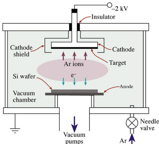
FIGURE 28.4. Sputtering system.
