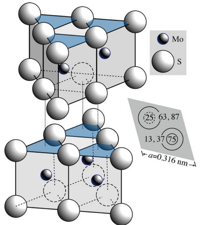
FIGURE 6.14. Crystal structure of molybdenite. S ions stack AABB, whereas Mo ions occupy half the trigonal prisms in each S “sandwich”.
