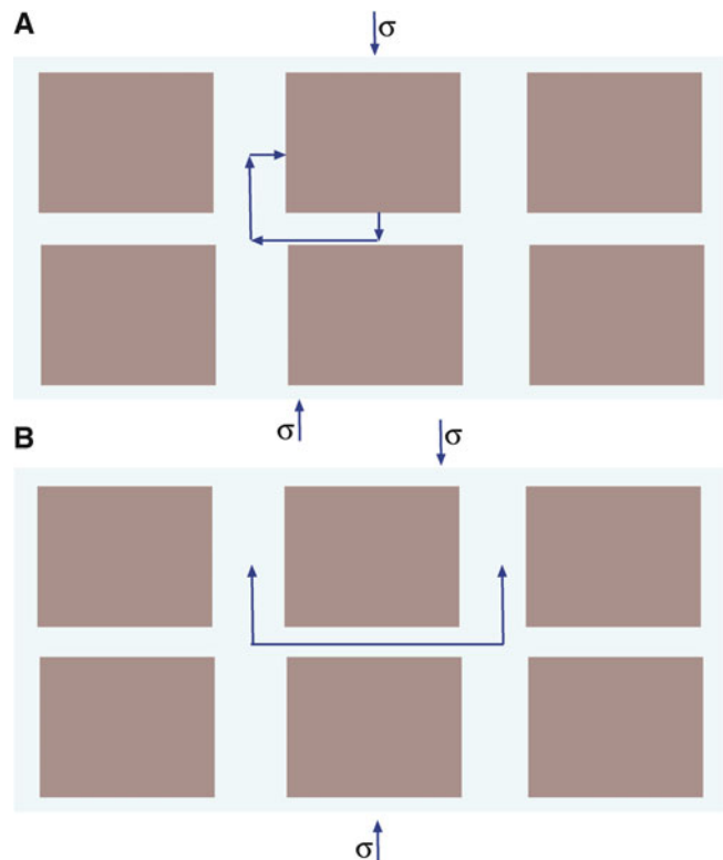
FIGURE 17.17. Dissolution-precipitation mechanism that could be operative in ceramics containing a glassy phase at the grain boundary.
