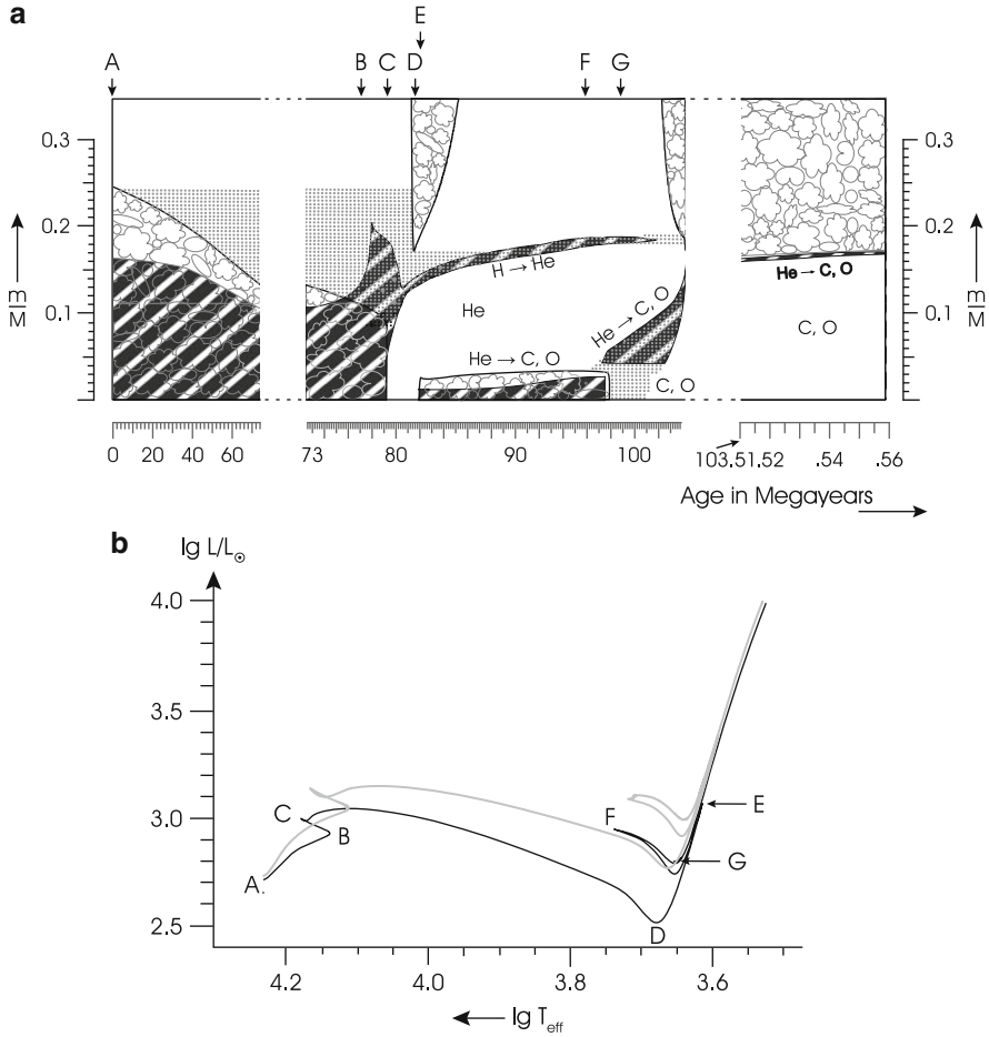
Fig. 31.2 (a) The evolution of the internal structure of a star of 5M_\odot of Population I. The abscissa gives the age (in units of 10^6 years) since the beginning of the evolution on the main sequence. Each vertical line corresponds to a model at a given time. The different layers are characterized by their values of m/M . “Cloudy” regions indicate convective areas. Heavily hatched regions indicate where the nuclear energy generation ( \epsilon_{\text{H}} or \epsilon_{\text{He}} ) exceeds 10^2 \text{ erg g}^{-1} \text{ s}^{-1} . Regions of variable chemical composition are dotted. The letters A . . . G above the upper abscissa indicate the corresponding points in the evolutionary track, which is plotted in Fig. 31.2 (b) with a solid line. The grey line in the Hertzsprung-Russell diagram shows the evolution of a star of the same mass and composition, but with convective overshooting included
