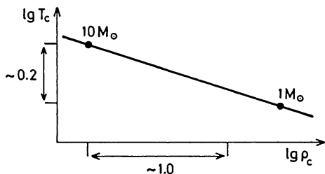
Fig. 20.2 The central values of T and \rho (both logarithmic) for homologous main-sequence stars of various M . The slope corresponds to a temperature sensitivity \nu typical for CNO burning
