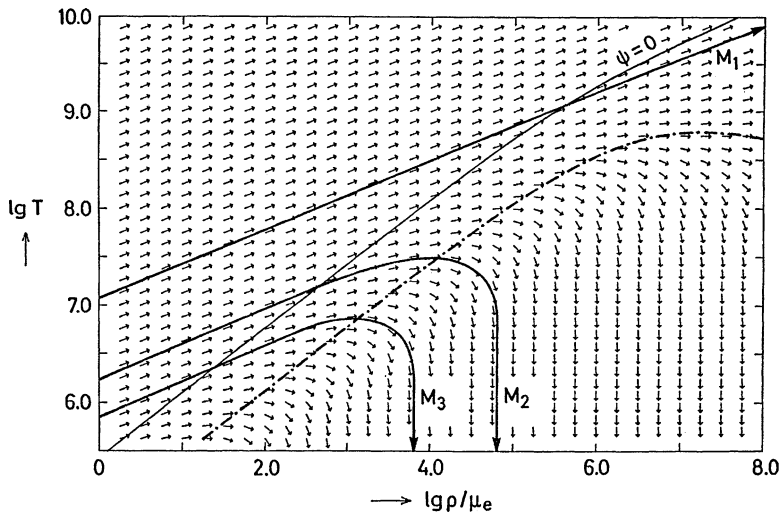
Fig. 28.2 Temperature T (in K) over density \rho/\mu_e (in \text{g cm}^{-3} ) with the vector field and the lines \psi = 0 and \alpha = 3/4 as in Fig. 28.1. The heavy lines give the “evolutionary tracks” of the centres of three homogeneously contracting stars of different masses. Mass M_1 is so large that the evolution is not remarkably influenced by degeneracy, and the centre continuously heats up during contraction. For mass M_2 (< M_1) degeneracy becomes important in the centre, and consequently a homologous contraction cannot bring the central temperature above a few 10^7 K (which is not sufficient to start helium burning). Mass M_3 (< M_2) while contracting will start to cool off even before the temperature of hydrogen burning is reached
