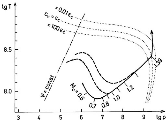
Fig. 35.4 Temperature T (in K) and density \rho (in \text{g cm}^{-3} ) in the CO core of a 3M_{\odot} star after central helium burning. The solid line gives the evolution of the centre with increasing core mass M_c (in M_{\odot} ). The carbon flash starts at about M_c = 1.39M_{\odot} when the energy production by carbon burning ( \epsilon_c ) exceeds the neutrino losses ( \epsilon_v ). Some lines of constant ratio \epsilon_v/\epsilon_c are dotted . The broken lines show the T stratification in the core for two consecutive stages; neutrino losses have produced a maximum of the temperature outside the centre (After Paczyński 1971)
