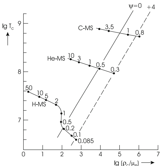
Fig. 23.3 Central temperature T_c (in K) and central density \rho_c/\mu_e ( \rho_c in \text{g cm}^{-3} , \mu_e = molecular weight per electron) of the models on the hydrogen, helium, and carbon sequences of Fig. 23.1. The labels along the lines give the stellar mass M (in M_{\odot} ). The dashed lines indicate constant degeneracy parameters \psi of the electron gas
