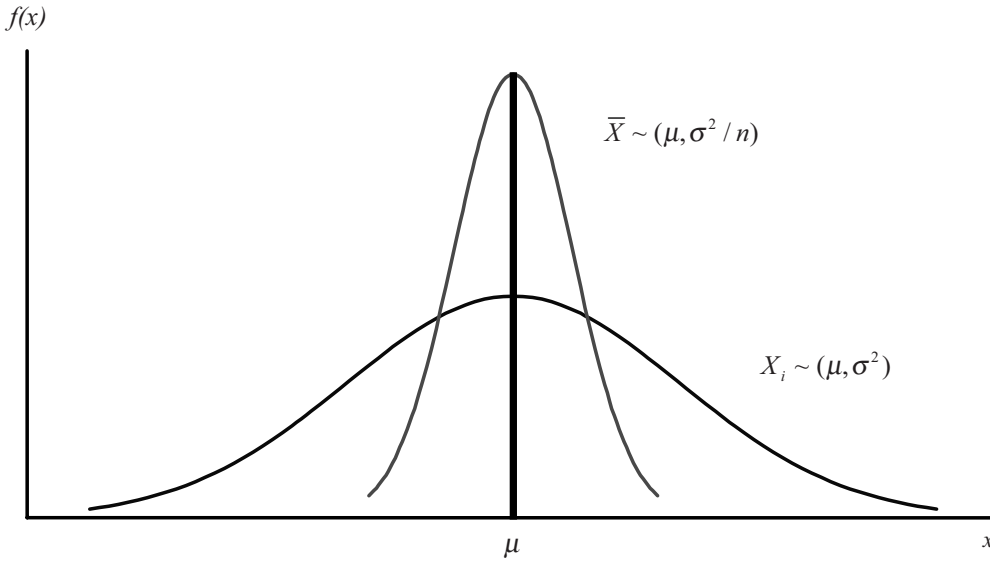
Figure 2.1 Efficiency Comparisons
