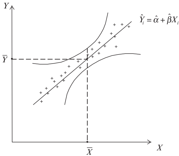
Figure 3.5 95% Confidence Bands
