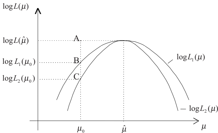
Figure 2.6 Wald Test
