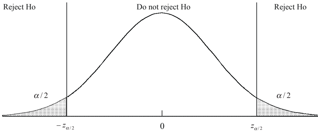
Figure 2.5 Critical Values
