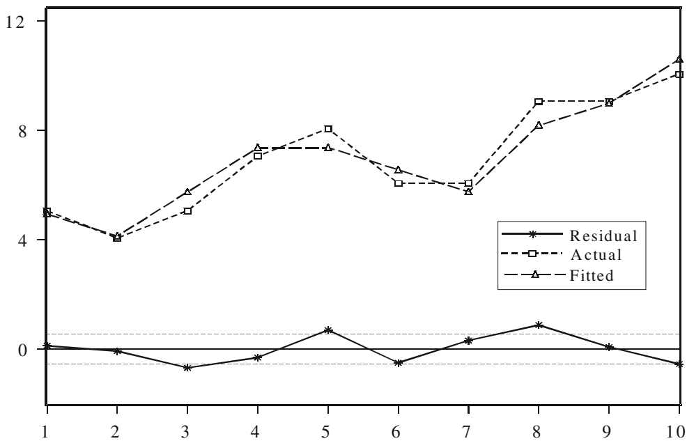
Figure 3.8 Residual Plot
