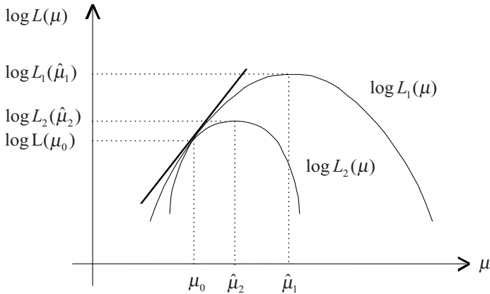
Figure 2.7 LM Test
