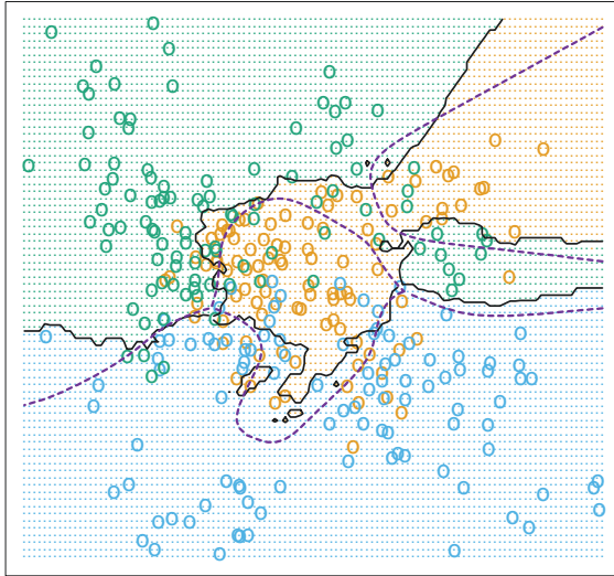
15-Nearest Neighbors
