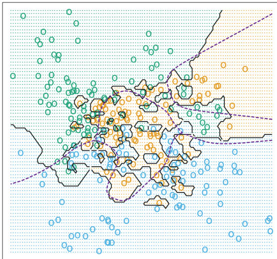
1-Nearest Neighbor
